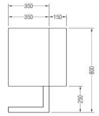
SIDE ELEVATION
