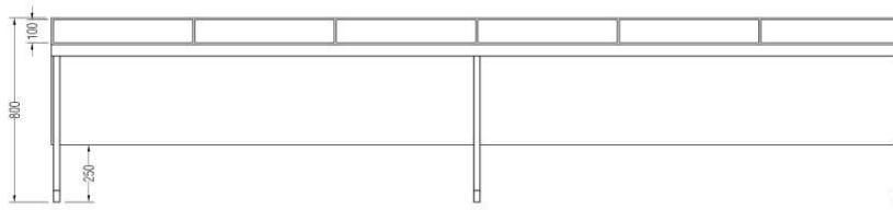
REAR ELEVATION
