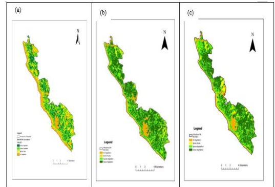
Figure 5: NDVI Analysis for Hikkaduwa DS. 2005 (a), 2014 (b), 2024 (c).
