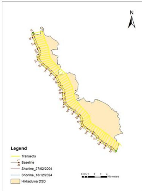
Figure 4: Change the Shoreline in Hikkaduwa DS from 2004-2024
