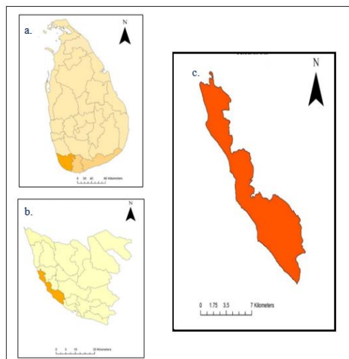
Figure 1: Study Area. Location of Galle District in Sri Lanka (a), Location of Hikkaduwa DSD in Galle District (b), Hikkaduwa DSD (c).
